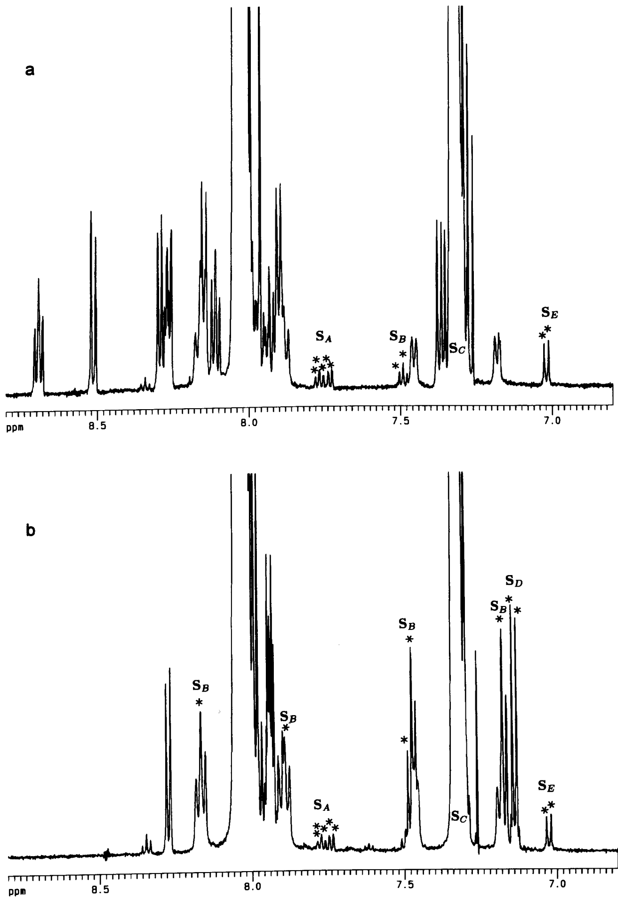
Figure 9 Expanded ^1\text{H} n.m.r. spectra for the ring proton resonances of samples 3a (a) and 3b (b). Signals of defect structures are marked by *
